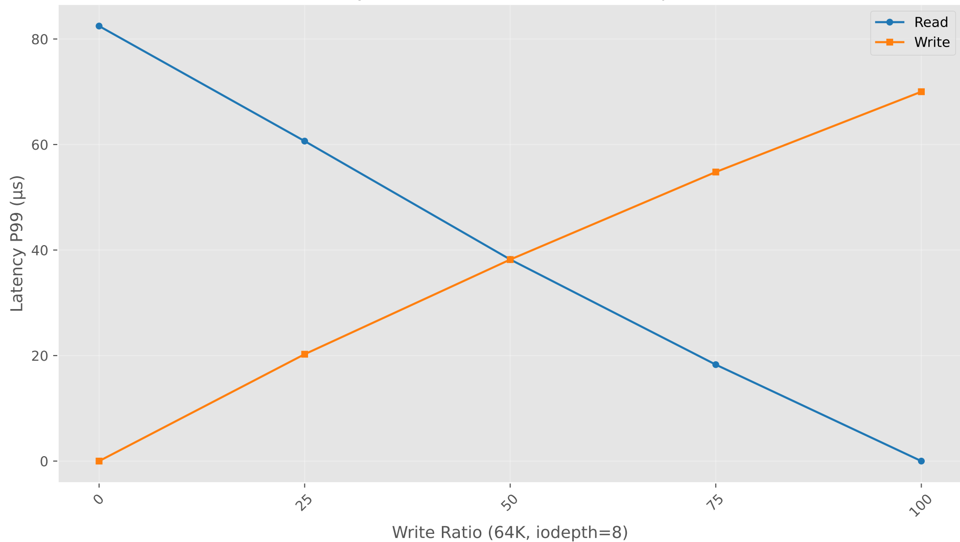
Latency P99 vs Write Ratio (64K, iodepth=8)
